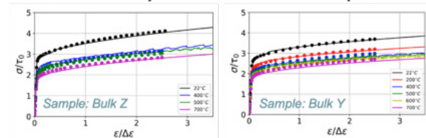
Figure 5. Temperature-dependent uniaxial stress-strain for different printed (symbols: simulations; solid lines: experiments).
