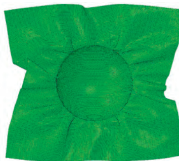
Figure 3. FEM deformation of a square fresh prepreg sheet during forming using and spherical indenter.
