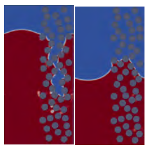
Figure 8. Fluid dynamics simulation of the flow propagation process at the micro level including viscous and capillary forces.
