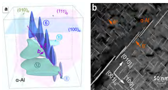
Figure 2. (a) Multiscale simulation of the nucleation and growth of \theta' (Al 2 Cu) precipitates on dislocations during high temperature aging of an Al-Cu alloy. (b) Transmission electron microscopy micrograph showing the formation of a staircase structure of \theta' precipitates on a dislocation. From H. Liu, B. Bellón, J. LLorca. Acta Materialia 132, 611-626, 2017.
