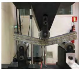
Figure 1. Fiber metal laminate (steel and glass) manufactured by UPM subjected to three-point bending (courtesy of Prof. Suárez Bermejo).
