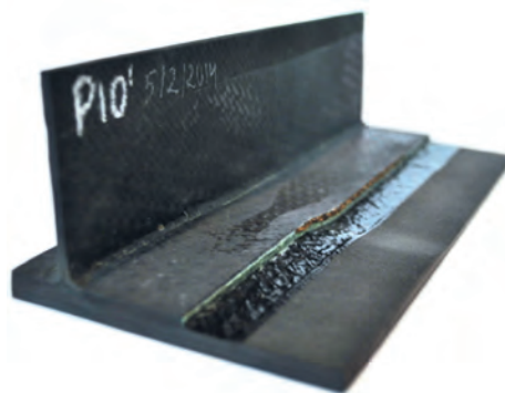
Figure 9. Detail of a stringer-skin integration manufactured by resin transfer moulding RTM.
