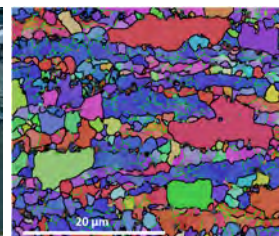
Figure 3. EBSD map of a steel after heat treatment.
