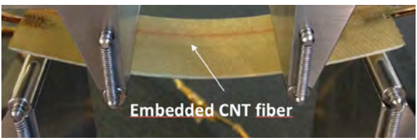
Figure 10. Four point bending tests of a composite material laminate with embedded CNT fiber for strain analysis.
